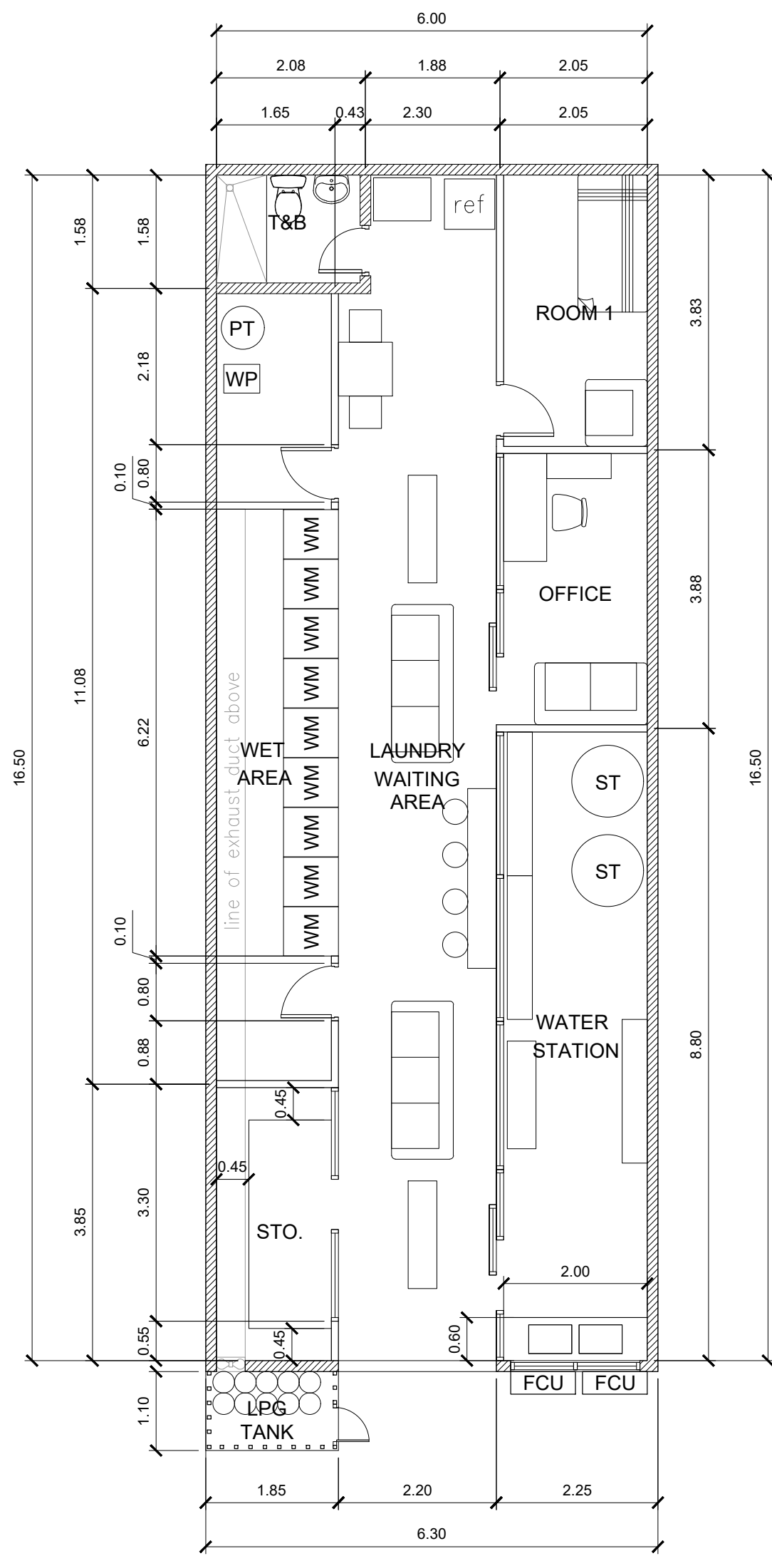
2 FURNITURE LAYOUT A-02 SCALE: 1:75 MTS.
