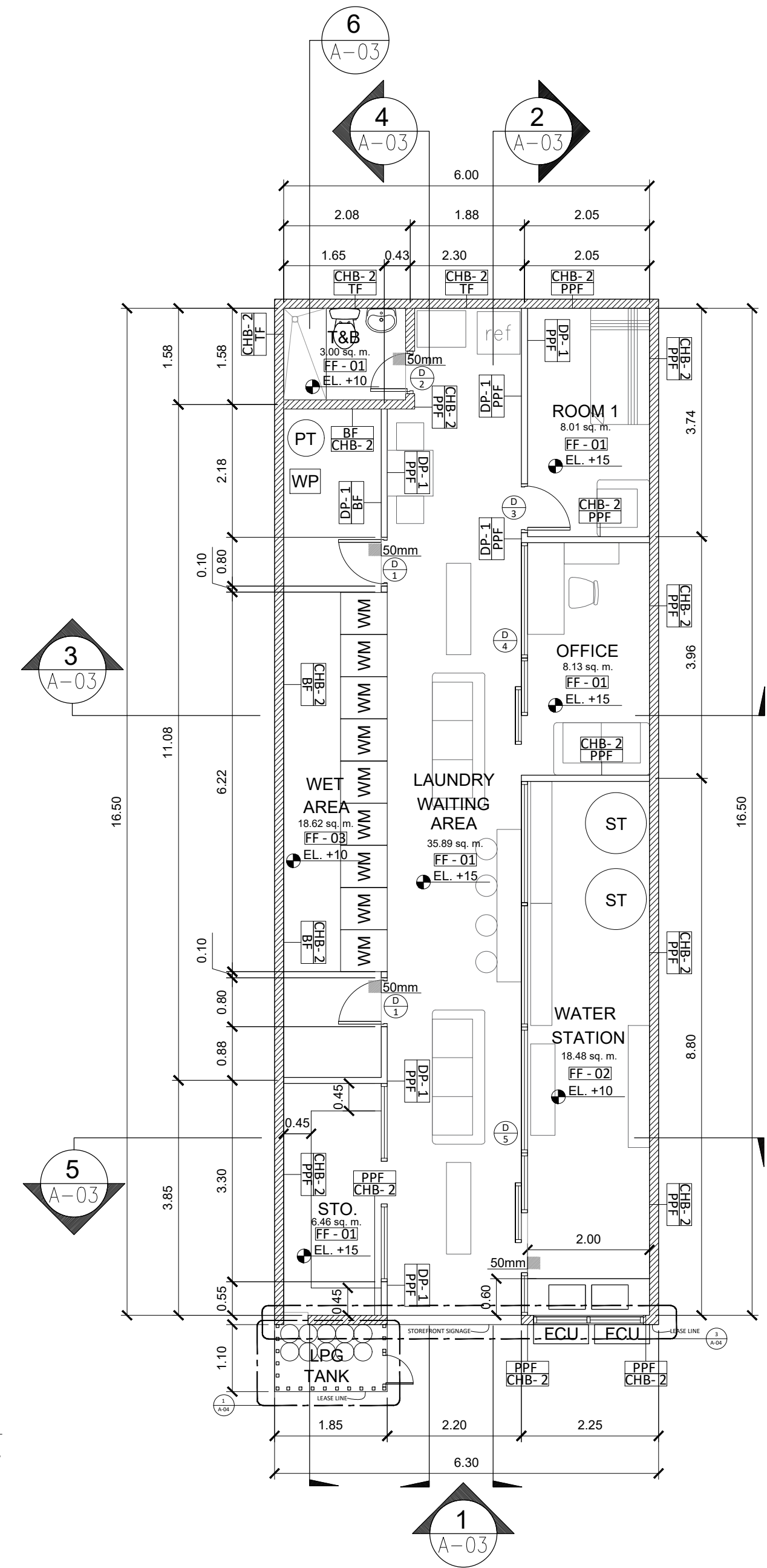
4 GROUND FLOOR PLAN A-02 SCALE: 1:75 MTS.
