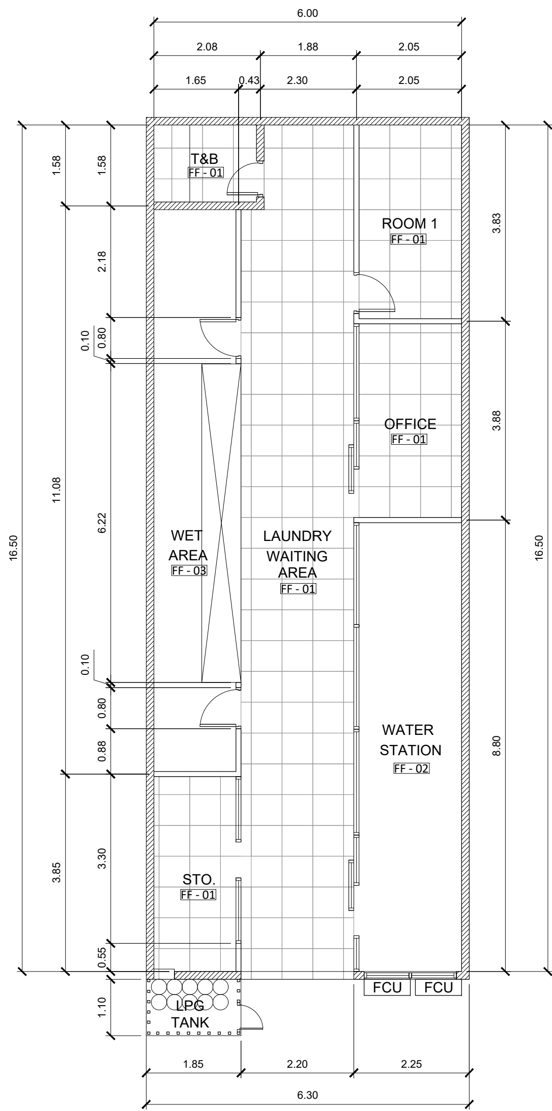
1 FLOOR FINISH LAYOUT A-02 SCALE: 1:75 MTS.
