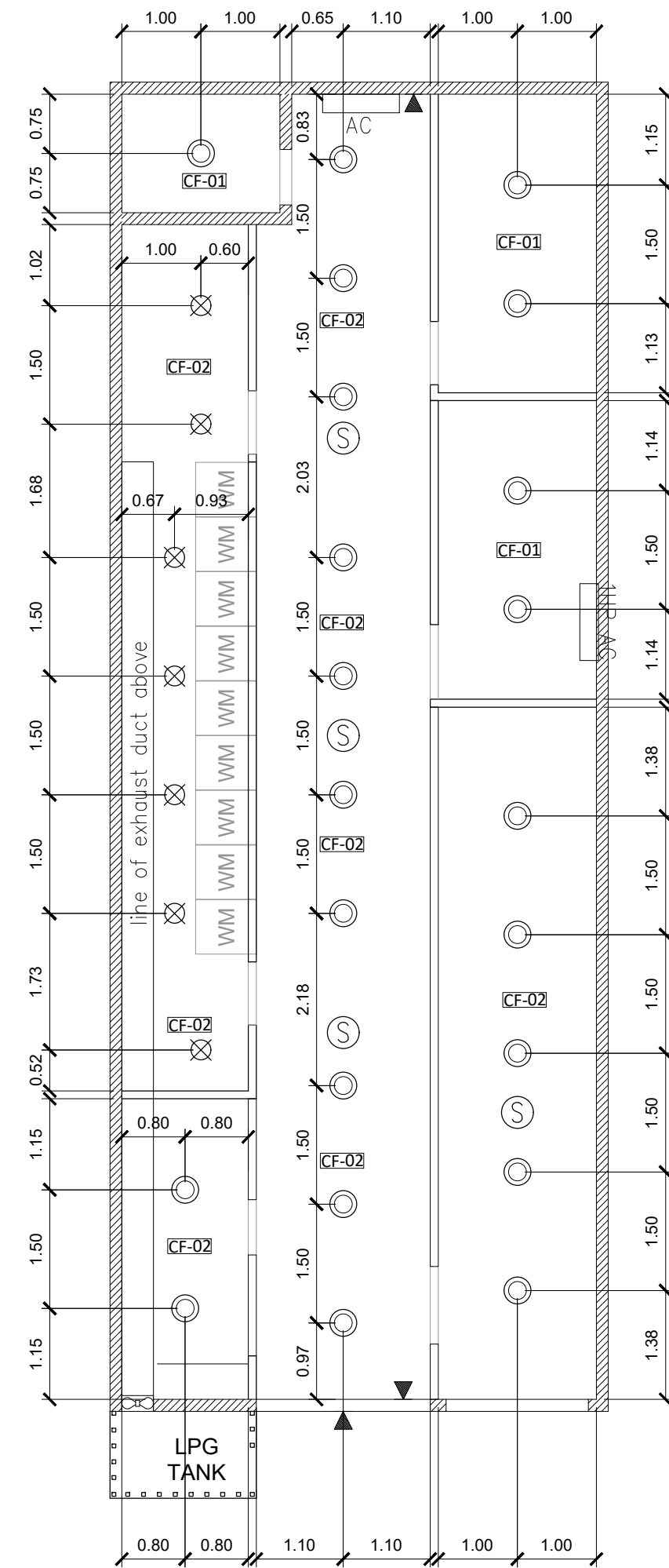
3 REFLECTED CEILING PLAN A-02 SCALE: 1:75 MTS.
